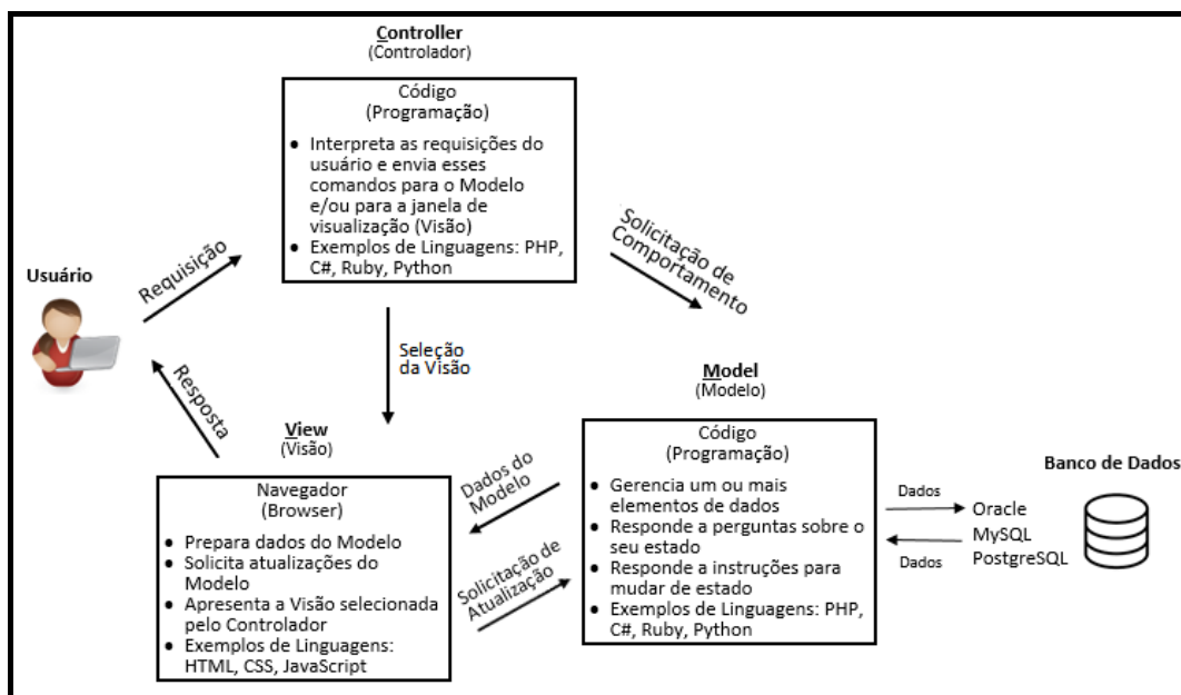
Figura 1: Model-View-Controller
